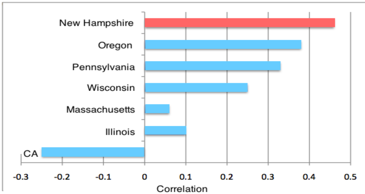
Figure 2. Primary Support for Opposition-Party Nominee and General Election Vote, 1952-2008.
