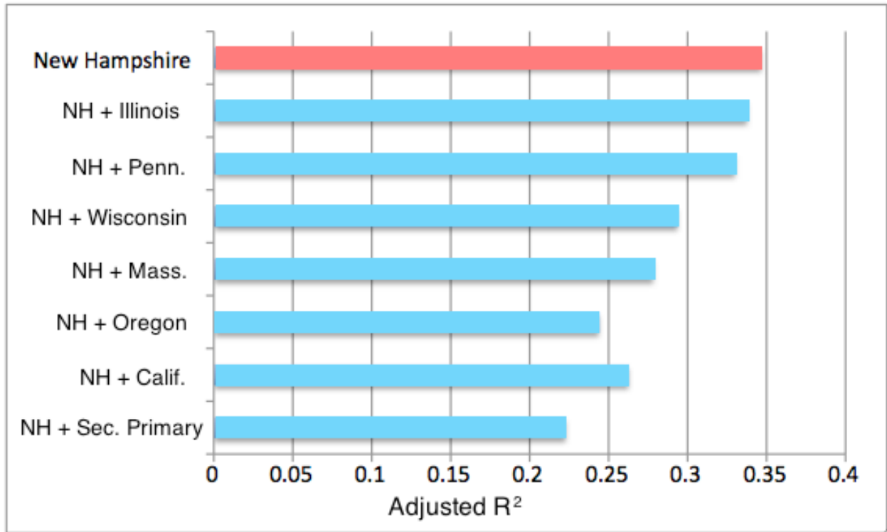
Figure 3. The Predictive Power of Primaries: New Hampshire and New Hampshire Plus (For Incumbent and Opposition-Party Nominees)
