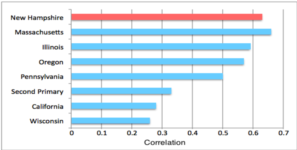
Figure 1. Primary Support for Incumbent-Party Nominee and General Election Vote, 1952-2008
