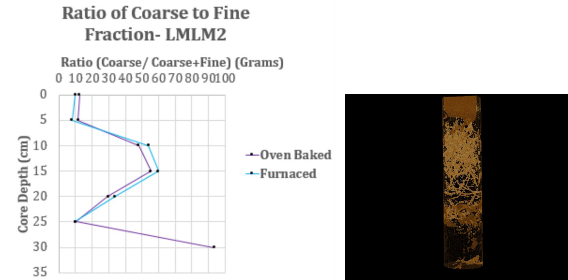
Figure 5 & 6 (above). LMLM2: As seen by Figure 5, the LMLM2 core has more fine material in its upper layers and more coarse material in its lower layers, particularly at 15 cm and 30 cm. Which, is consistent with CT data and calculations based on sediment deposition, which indicates these larger particles were brought in by storms around 1907-1929 and 1973 (Figure 6: Maher, 2020).
