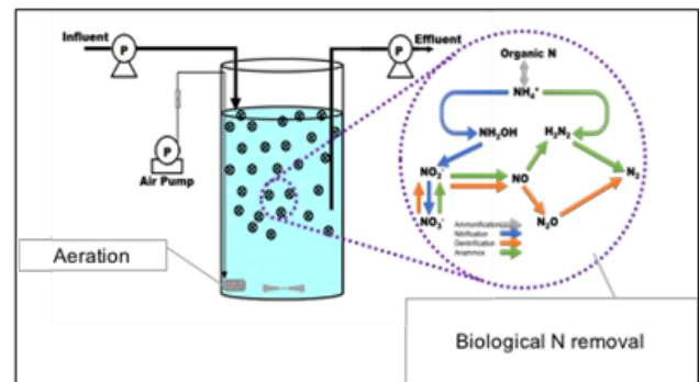
Figure 12 - MBBR-MBR
