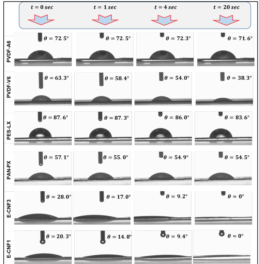
Figure 14 - Dynamic Contact Angle Measurements
