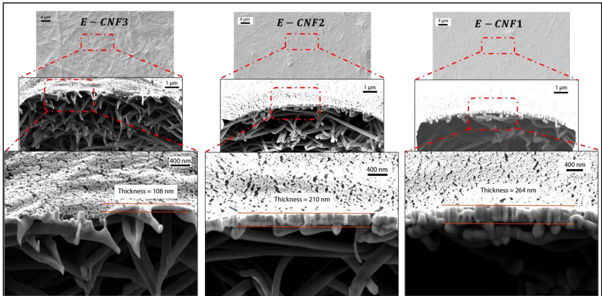
Figure 13 - Cross-Sectional SEM Images of the E-CNF1, E-CNF1, and E-CNF3 at Different Magnifications
