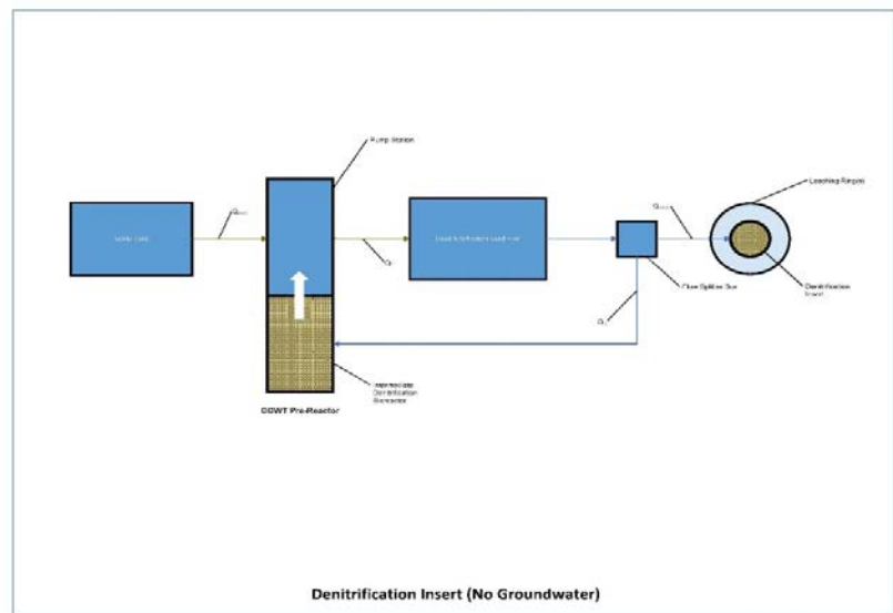
Figure 6 - NRB 2.0 Intermediate Bioreactor Process Schematic
